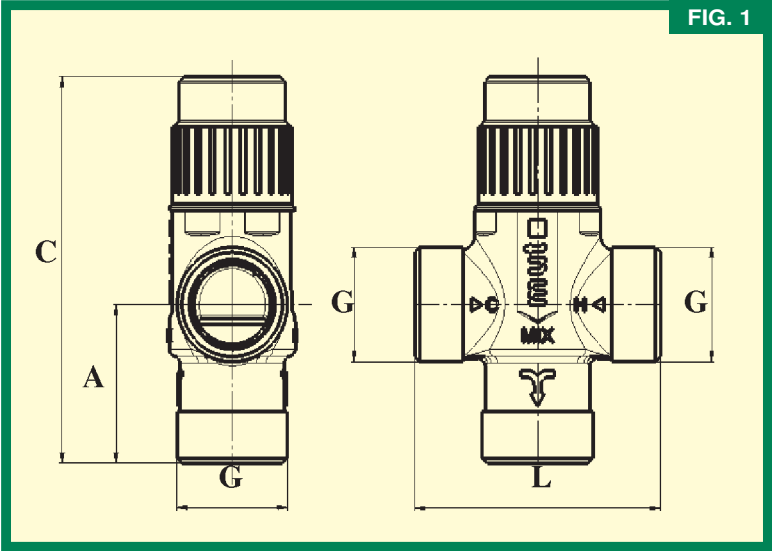
Fig. 1: dimensioni valvola TWR-RA / Fig. 1: TWR-RA valve dimensions Abb. 1: Dimensionen Ventile TWR-RA / Dessin 1: Dimensions valve TWR-RA / Fig.1: Dimensiones valuvulas TWR-RA
